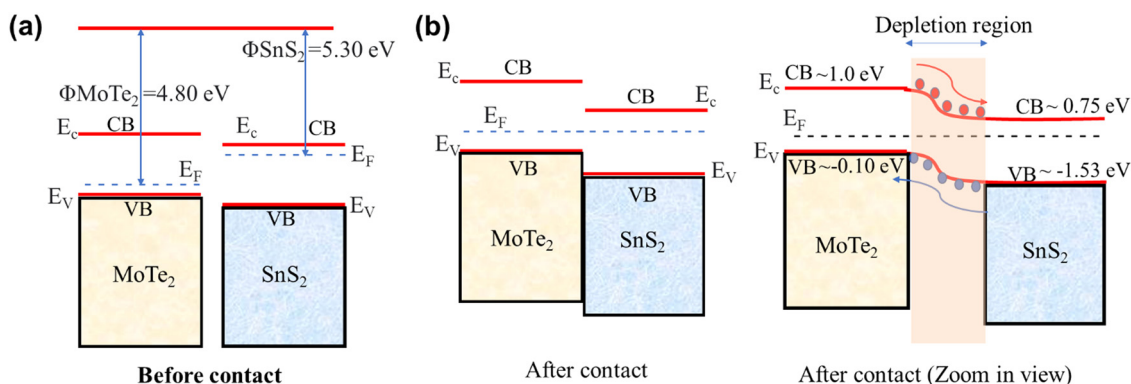
Fig. 5 Schematic illustration of the band diagram for the p-MoTe 2 /n-SnS 2 structure-based diode at V_{bg} = 0\text{V} . (a) Schematic signifies the band diagram of a p-MoTe 2 /n-SnS 2 diode before connection, and (b) symbolizes the diode after connection.
