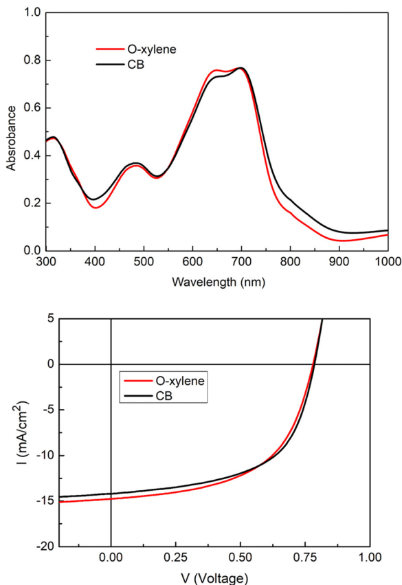
Fig. 3 Absorption spectra and I - V curves of PTB7-Th:AzaTk blend film deposited from o -xylene and chlorobenzene solutions.
