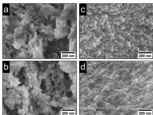
Fig. 5 SEM images (100k magnification) of (a) \text{nDUT-5:Eu}^{3+} , (b) \text{nDUT-5:Tb}^{3+} , (c) \text{nMOF-253:Eu}^{3+} and (d) \text{nMOF-253:Tb}^{3+} .
