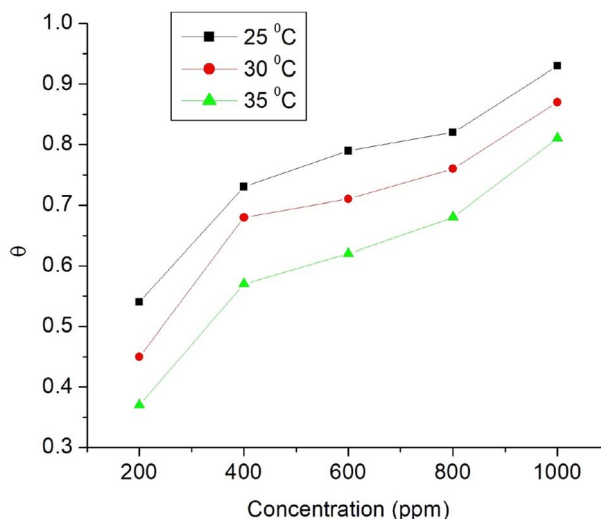
Fig. 11 Henry adsorption isotherm ( \theta ) versus concentration of \text{Co}_3\text{O}_4\text{@PPy} NCs at 25, 30, and 35 °C.
