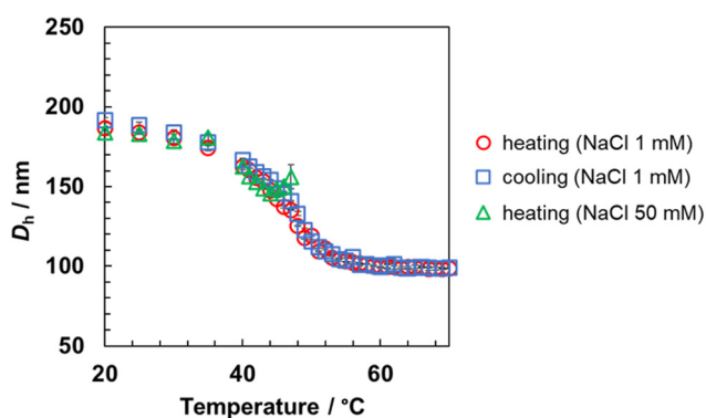
Fig. 2 Temperature dependence of the hydrodynamic diameter ( D_h ) of the ND10 microgels in the presence of different salt concentrations, as derived from the DLS measurements.
