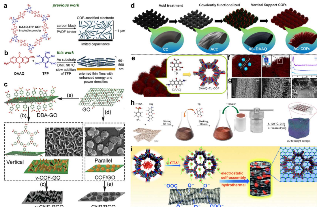
Fig. 11 (a) Structure of the hexagonal subunit of the DAAQ-Tp COF, which was previously prepared as a slurry, mixed with carbon black and a PVDF binder, for supercapacitor applications. (b) Solvothermal growth of the DAAQ-Tp COF as an oriented thin film on Au electrodes. Reprinted from ref. 97. Copyright 2015, American Chemical Society. (c) Schematic illustration of the preparation of v-COF-GO and COF/GO to produce carbon nanosheets oriented vertical or parallel to the rGO surface. Reprinted from ref. 99. Copyright 2018, Wiley-VCH GmbH. (d) Schematic diagram of the functionalized AC-COFs. (e) Synthesis and structural characterization of COFs. (f) Schematic illustration of electron transport in AC-COFs and PXRD patterns of the AC-COFs at different times. (g) SEM and cross-section images of AC-COFs at different time intervals. Reprinted from ref. 100. Copyright 2022, American Chemical Society. (h) Scheme of the synthetic procedure for the preparation of the COF/rGO aerogel. Reprinted from ref. 101. Copyright 2020, Springer Nature Limited (Creative Commons CC BY). (i) Scheme of the synthesis procedure for the DAAQ-COFs/GA composite. Reprinted from ref. 102. Copyright 2021, Royal Society of Chemistry.
