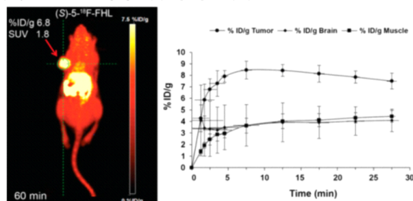
Scheme 7 (a) PET images at 10 min for U-87 xenograft-bearing mice with (S)-5-[[ ^{18}\text{F} ]]-FHL (24), (S)-5-[[ ^{18}\text{F} ]]-F \alpha MHL (25), (S)-4-[[ ^{18}\text{F} ]]-F \alpha ML (26), and 5-[[ ^{18}\text{F} ]]-FPregab (27). The orange arrow indicates the site of tumor. (b) In vivo dynamic PET imaging of (S)-5-[[ ^{18}\text{F} ]]-FHL in NSG mouse bearing U-87 xenograft tumor at 60 min after injection and time-activity curve of (S)-5-[[ ^{18}\text{F} ]]-FHL (24) in tumor, brain, and muscle over 30 min after injection, n = 3 . Images reproduced with permission from ref. 83, copyright 2019 the Society of Nuclear Medicine and Molecular Imaging.
