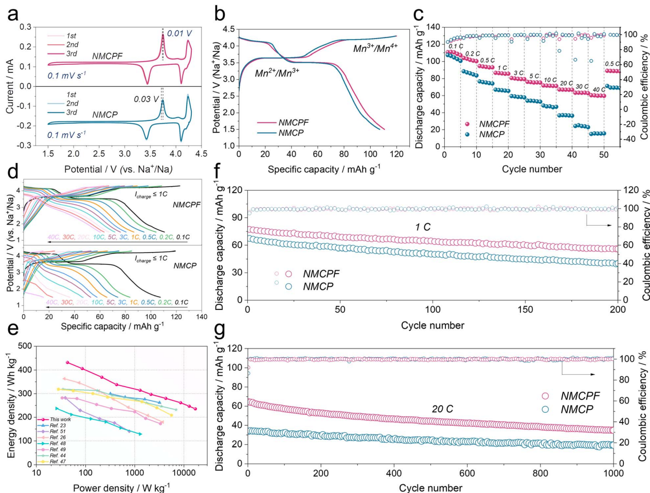
Fig. 4 Electrochemical capabilities within 1.5–4.3 V. (a) CV curves at 0.1 mV s -1 . (b) Initial charge/discharge curves at 0.1C (1C = 110 mA h g -1 ). (c) Rate properties. (d) Charge/discharge profiles at various rates. (e) Ragone plot. Cycling capabilities at (f) 1C and (g) 20C.
