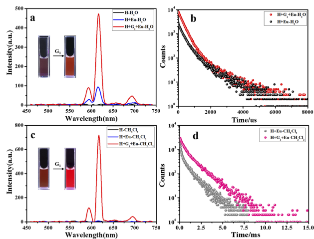
Fig. 4 Luminescent emission spectra of (a) H (black line), H / Eu 3+ (blue line), and H / Eu 3+ / G 1 (red line), and time-resolved photoluminescence decay curves of (b) H / Eu 3+ (black line) and H / Eu 3+ / G 1 (red line) in aqueous solution at 298 K. (c) Corresponding emission and (d) time-resolved photoluminescence decay curves in CH 2 Cl 2 solution ([ H ] = 2.0 \times 10^{-5} \text{ M} ) at 298 K.
