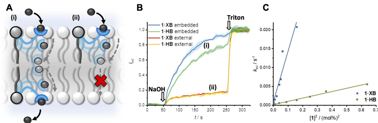
Fig. 2 (A) Relay anion transport. (B) Change in ratiometric emission, I_{rel} ( \lambda_{em} = 510 nm; \lambda_{ex1} = 405 nm, \lambda_{ex2} = 460 nm), upon addition of a NaOH base pulse (5 mM) to POPC LUVs (31 \mu M) containing 1 mM HPTS, 100 mM internal and external NaCl, buffered with 10 mM HEPES at pH 7.0. (i) Data for relay transporter pre-incorporated during LUV preparation (0.25 mol% 1·XB with respect to lipid and 1 mol% 1·HB) and (ii) following external addition of 1 mol% relay transporter in DMSO (>95% membrane incorporation efficiency). (C) Concentration dependence of relay activity with pre-incorporated 1·XB and 1·HB, and linear relationship for the initial rate, k_{ini} with respect to [1]^2 .
