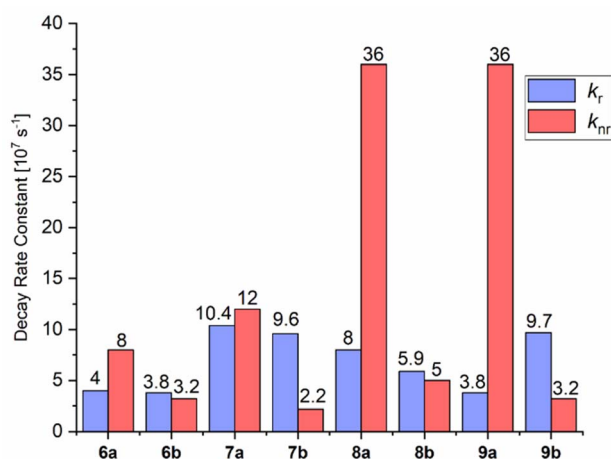
Fig. 8 Radiative ( k_{\text{r}} ) and non-radiative ( k_{\text{nr}} ) decay rate constants of compounds 6–9 in the solid state. The decay rate constants are determined according to k_{\text{r}} = 1/\tau_{\text{av\_amp}} = \Phi_{\text{F}}/\tau_{\text{av\_amp}} and k_{\text{nr}} = 1 - \Phi_{\text{F}}/\tau_{\text{av\_amp}} by using amplitude-weighted average lifetimes, according to Engelborghs et al. 50 The uncertainty analysis is not presented in this diagram for clarity (for k_{\text{r}} and k_{\text{nr}} in MeCN solutions at RT and a frozen glassy matrix in butyronitrile at 77 K, see Chapter 4 in the ESI†).
