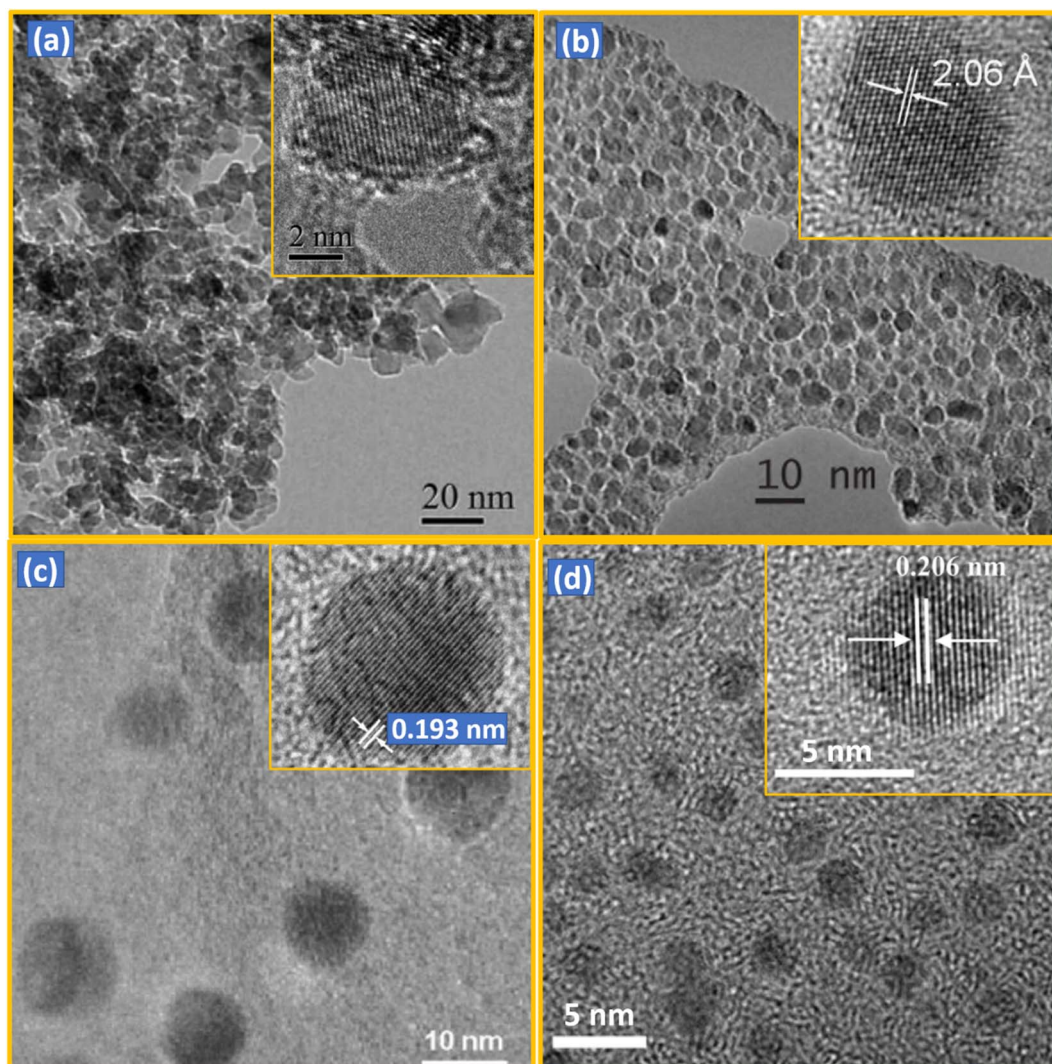
Fig. 3 TEM images of NDs synthesized by different methods: (a) detonation ( d = 4-5 nm), 116 (b) HPHT after fragmentation ( d = 2-7 nm; d_{\text{avg}} = 3.5 nm), 112 (c) CVD ( d = 1-10 nm), 57 and (d) laser ablation ( d_{\text{avg}} = 3.5 nm). 117 Low- and high (inset)-resolution images are provided. Reproduced with permissions from ref. 116 Copyright 2012 Royal Society of Chemistry, ref. 112 Copyright 2009 IOP Science, ref. 57 Copyright 2003 American Institute of Physics, and ref. 117 Copyright 2015 American Chemical Society.
