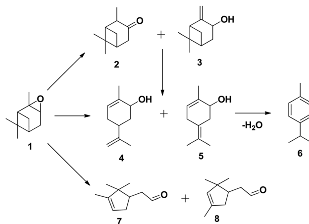
Scheme 17 Products of isomerisation of \alpha -pinene oxide; (1) \alpha -pinene oxide, (2) isopinocampheol, (3) pinocarveol, (4) trans -carveol, (5) 2-methyl-5-(propan-2-ylidene) cyclohex-2-enol, (6) p -cymene, (7) campholenic aldehyde and (8) fencholenic aldehydes. 10
