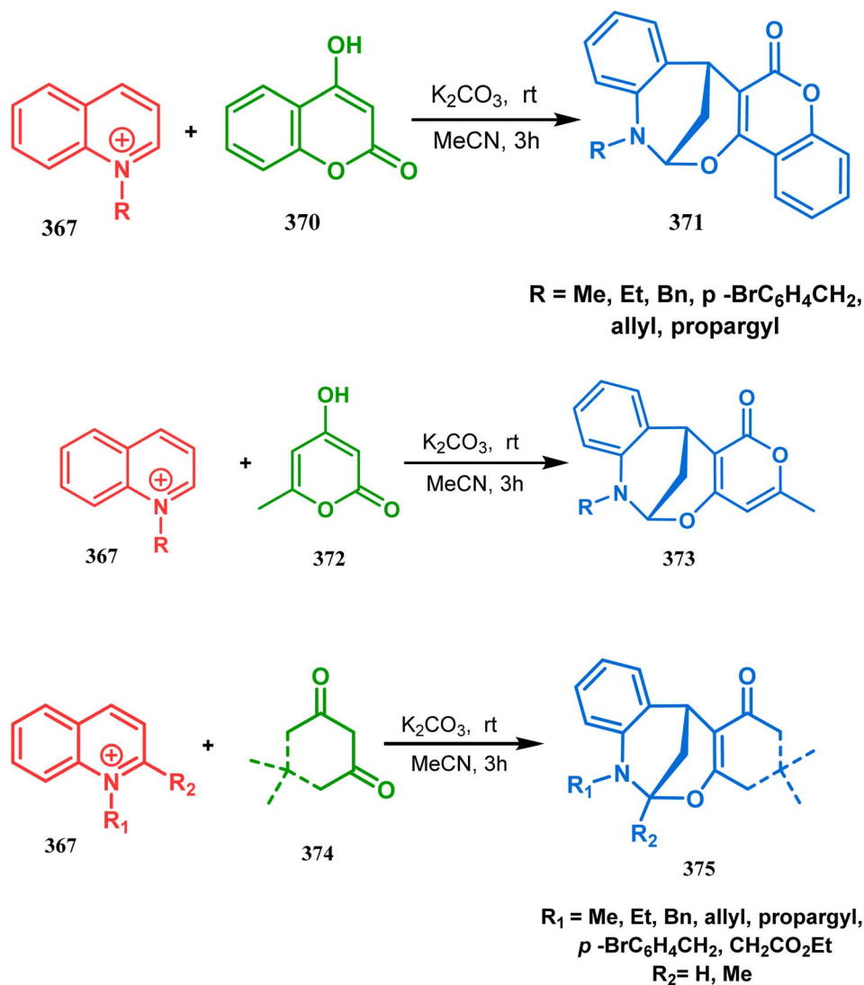
Scheme 85 (a) Synthesis of oxazabicyclo[3.3.1]nonane by the reaction of 4-hydroxycoumarin and N -alkylquinoliniums through tandem C-alkylation and intramolecular O-cyclization (b): synthesis of oxazabicyclo[3.3.1]nonane by the reaction of 4-hydroxy-pyrone derivative and N -alkylquinoliniums through tandem C-alkylation and intramolecular O-cyclization (c) synthesis of methylene-bridged benzoxazocines by the reaction of active methylene-containing 1,3-diketones and N -alkylquinoliniums through tandem C-alkylation and intramolecular O-cyclization.
