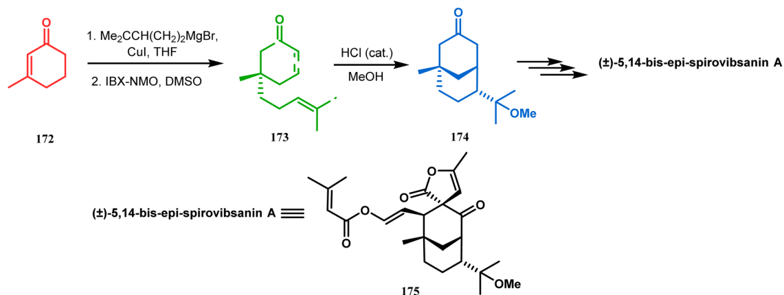
Scheme 34 Synthesis of (±)-5,14-bis- epi -spirovibsanin A containing the bicyclo[3.3.1]nonane core through intramolecular cation capture.
