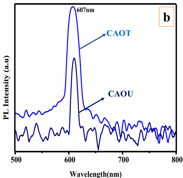
Fig. 9 (a) PL excitation spectrum. (b) PL emission spectra ( \lambda_{\text{ex}} = 350 nm) of the as-formed and calcined CAOT and CAOU NPs.
