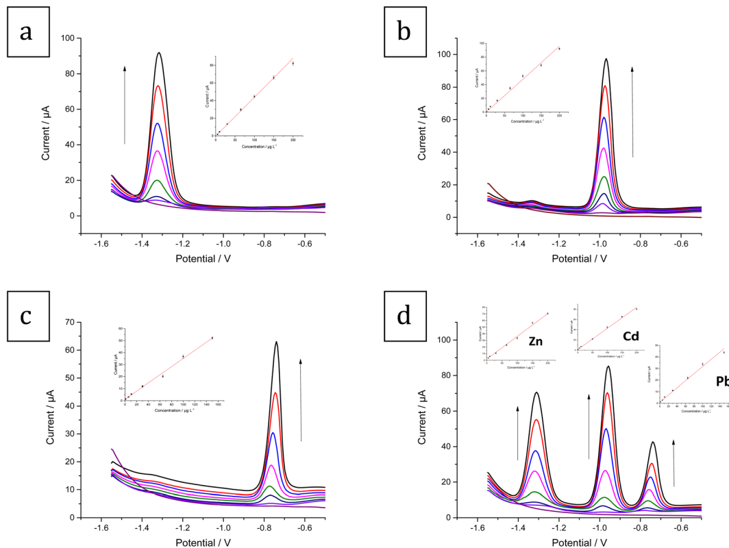
Fig. 11 SW-ASV results and calibration for (a) Zn 2+ (0 (blank), 5, 10, 30, 65, 100, 150, 200 \mu\text{g L}^{-1} ) (b) Cd 2+ (0 (blank), 1, 6, 11, 30, 65, 100, 150, 200 \mu\text{g L}^{-1} ) (c) Pb 2+ (0 (blank), 1, 6, 11, 30, 65, 100, 150 \mu\text{g L}^{-1} ) (d) the three metal ions simultaneously: Zn 2+ (0 (blank), 5, 10, 30, 65, 100, 150, 200 \mu\text{g L}^{-1} ), Cd 2+ (0 (blank), 1, 6, 11, 30, 65, 100, 150, 200 \mu\text{g L}^{-1} ), and Pb 2+ (0 (blank), 1, 6, 11, 30, 65, 100, 150 \mu\text{g L}^{-1} ) in ABS pH 5.6, \text{dp } E = -1.55 \text{ V} and \text{dp } t = 180 \text{ s} at the Bi-Sb/CPE.
