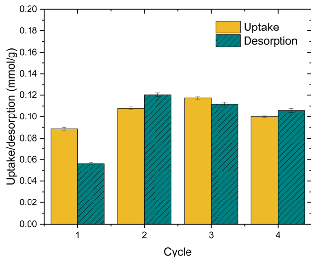
Fig. 11 A total uptake of \text{Zr}(\text{Sb})\text{O}_2 after the several successive load (10 mM \text{Na}_2\text{SO}_4 , 1 mM \text{KIO}_3 pH 6), desorption (0.1 M NaOH) and regeneration (0.1 M HCl) cycles.
