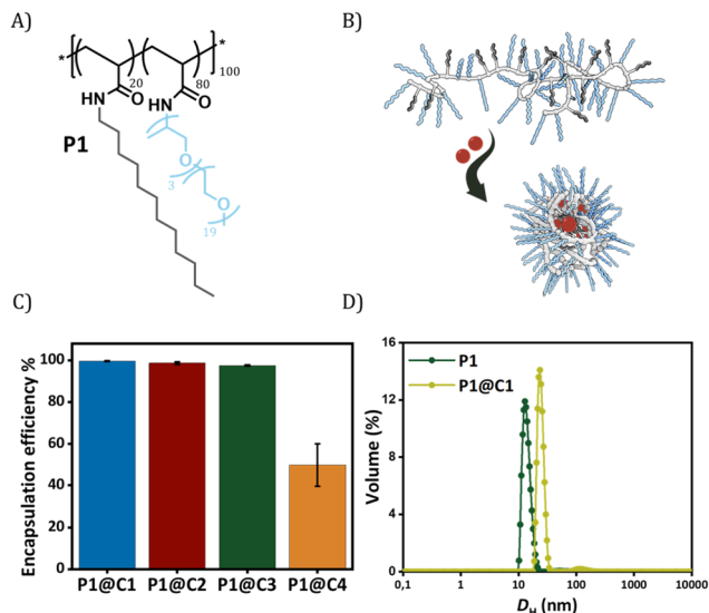
Fig. 2 (A) Chemical structure of amphiphilic random copolymer P1 , DP = 100, \bar{D} = 1.21; (B) representation of the encapsulation of catalysts C1–C4 (red spheres) in the hydrophobic interior of polymeric nanoparticles; (C) encapsulation efficiency of the dirhodium carboxylate catalysts C1–C4 in polymeric nanoparticles calculated from the leached-out rhodium using ICP-OES. [ P1 ] = 1 mg mL −1 , P1 : C = 1 : 5 (molar ratio), [Rh] = 10 mg L −1 before filtration. The results for the encapsulation efficiency are the average of three independent measurements; (D) volume distribution of the hydrodynamic diameter D_H of P1 and P1@C1 nanoparticles ([ P1 ] = 1.0 mg mL −1 , T = 20 °C, [ P1 ] : [ C1 ] = 1 : 5 (molar ratio)) monitored using DLS measurements.
