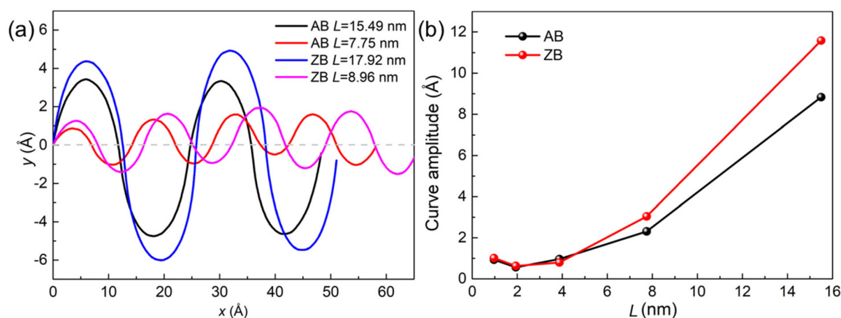
Fig. 3 (a) The fitted Fourier curve for the structural trajectory of the MoSSe/WSSe heterostructure superlattice and (b) the amplitude value of the Fourier curve versus L .
