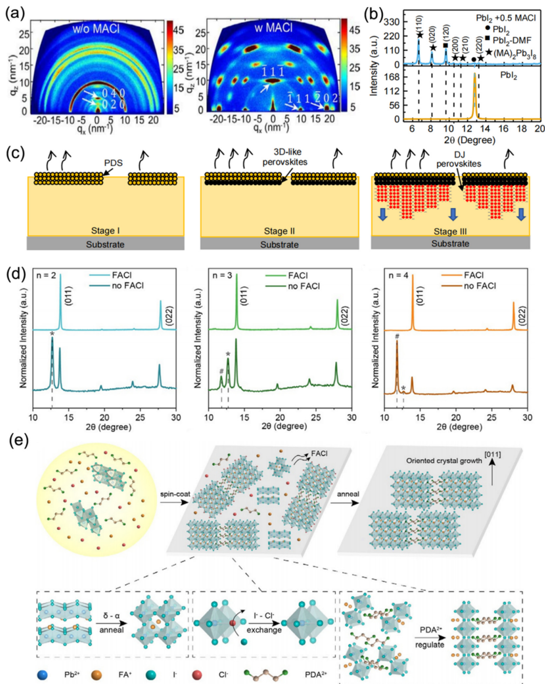
Fig. 13 (a) GIWAXS images of (\text{PXD})(\text{MA})_2\text{Pb}_3\text{I}_{10} perovskite films without and with MACl additive. (b) XRD curves of perovskite films without and with MACl additive. (c) Schematic diagram of the crystallization process for DJ phase perovskite films with MACl additive. Reproduced with permission from ref. 96. Copyright 2020 Wiley-VCH. (d) XRD patterns of perovskite films with different n values prepared with and without FAcI additive. (e) Schematic illustration of the mechanism of perovskite film growth with FAcI additive. Reproduced with permission from ref. 97. Copyright 2020 Wiley-VCH.
