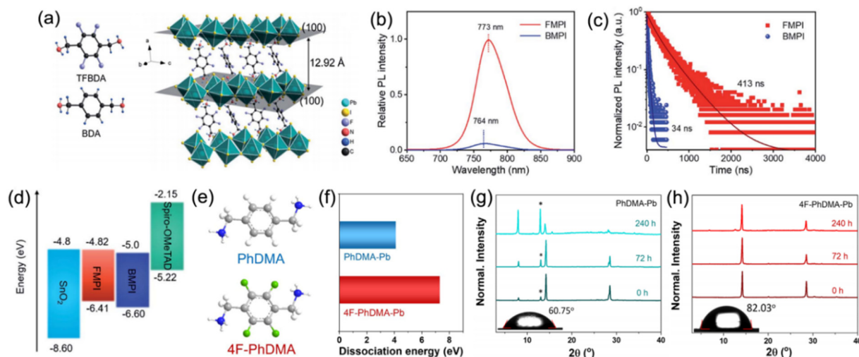
Fig. 8 (a) Chemical structures of TFBDA 2+ and BDA 2+ cations, and the crystal structure of (TFBDA)PbI 4 . (b) PL spectra and (c) PL decay of TFBDA 2+ and BDA 2+ based perovskite films. (d) Energy band alignment of TFBDA 2+ and BDA 2+ based quasi-2D PSCs. The TFBDA based perovskite is named FMPI, while the BDA based perovskite is named BMPI. Reproduced with permission from ref. 90. Copyright 2021 Royal Society of Chemistry. (e) Chemical structure of PDMA 2+ and 4F-PDMA 2+ cations. (f) Dissociation energy of PDMA-Pb and 4F-PDMA-Pb based perovskites. XRD patterns of (g) PDMA-Pb and (h) 4F-PDMA-Pb based quasi-2D perovskite films exposed to an ambient atmosphere. Reproduced with permission from ref. 88. Copyright 2021 American Chemical Society.
