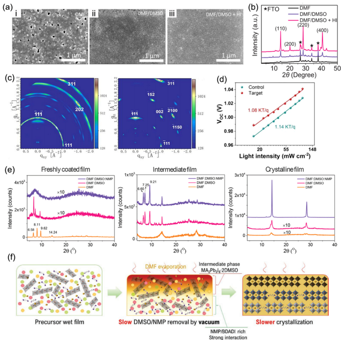
Fig. 10 (a) SEM images and (b) XRD patterns of (3AMP)(MA 0.75 FA 0.25 ) 3 Pb 4 I 13 films processed in DMF, DMF/DMSO, and DMF/DMSO/HI solvents. Reproduced with permission from ref. 20. Copyright 2019 Wiley-VCH. (c) GIWAXS data of the ThDMA-based DJ perovskite films: control (with DMF solvent, left) and target films (with optimized DMF/DMSO binary solvent, right). (d) Relation of the V_{oc} versus light intensity for ThDMA-based DJ perovskite control and target films. Reproduced with permission from ref. 113. Copyright 2020 American Chemistry Society. (e) XRD patterns of perovskite films synthesized with different solvents. (f) Schematics of vacuum-assisted crystallization processes for DJ perovskites synthesized with the ternary solvent DMF:DMSO:NMP. Reproduced with permission from ref. 125. Copyright 2022 Wiley-VCH.
