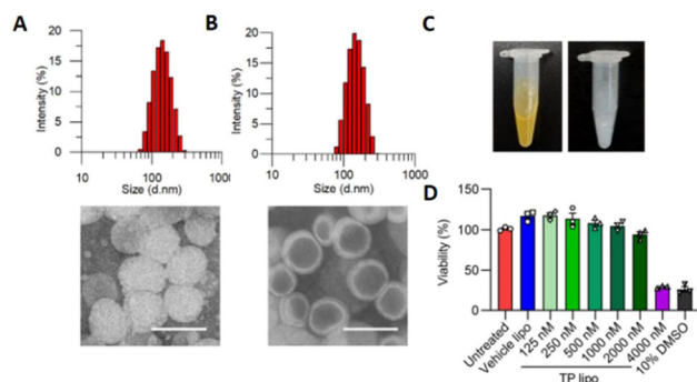
Fig. 5 Characterization of TP lipo. (A and B) TEM images of TP lipo (left) and vehicle lipo (right). The sizes are approximately 134.3 nm for TP lipo and 142.0 nm for vehicle lipo, scale bar = 200 nm. (C) Images of TP lipo and Vehicle lipo. (D) The effects of vehicle lipo, TP lipo at various doses, and 10% DMSO on the viability of Vero E6 cells. TP lipo: tripterin liposomes. Reproduced from ref. 75 with authorization. Copyright 2019, Springer Nature.
