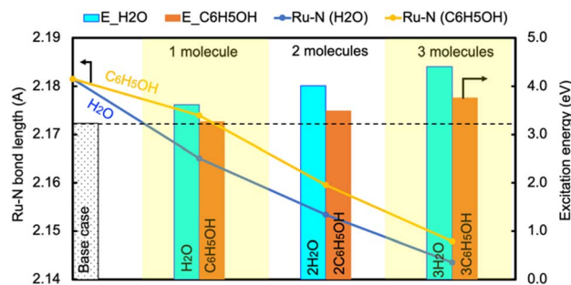
Fig. 5 The change in the excitation energy to excite an electron from the Fermi level to the LUMO of NH 3 and the Ru–N bond length as the number of H 2 O/C 6 H 5 OH molecules increases.
