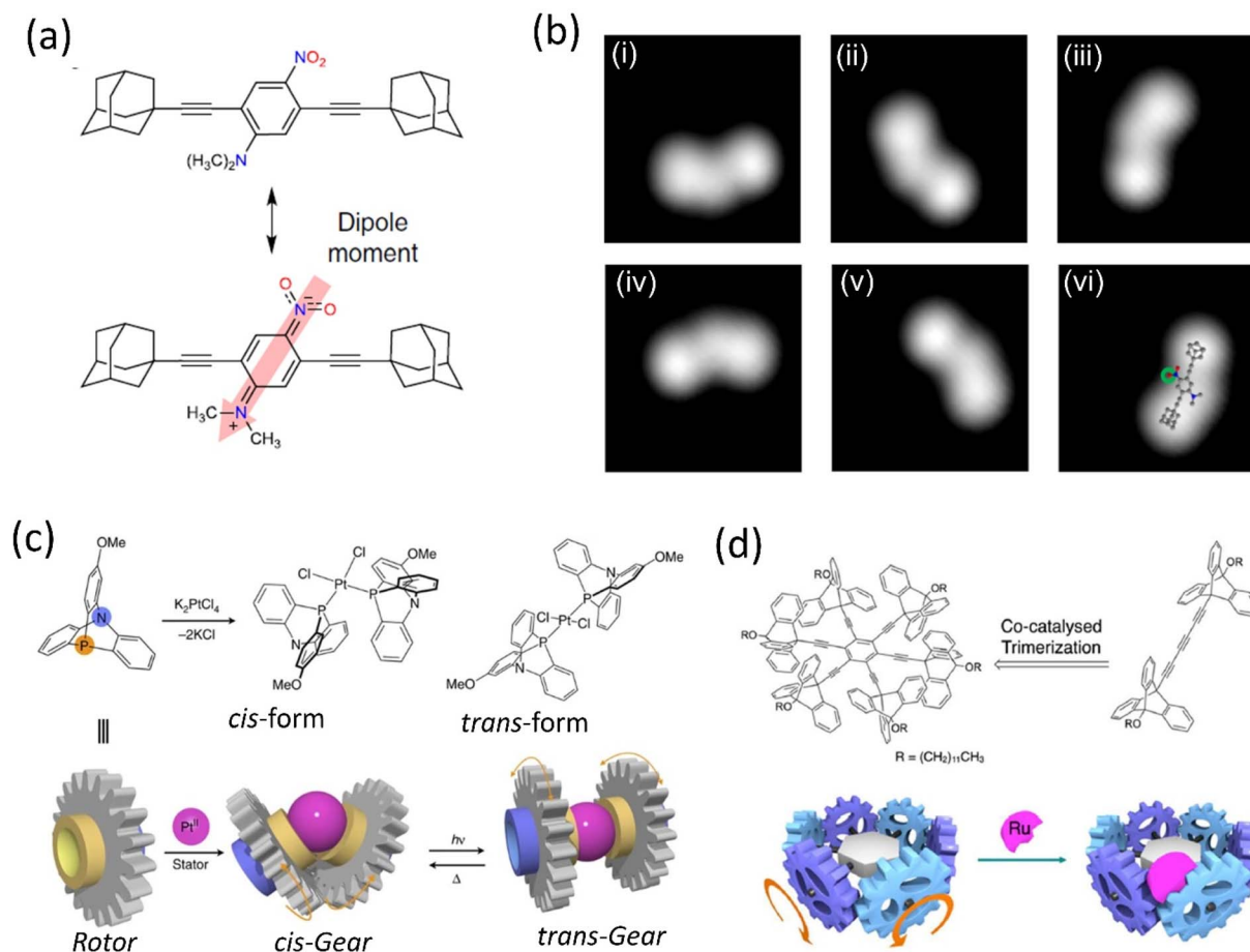
Fig. 7 (a) Chemical structure of polar motor. (b) (i)–(vi) STM images of the molecule showing clockwise rotation upon applied voltage pulse. Reproduced with permission. 150 Copyright 2019, The Authors, published by Springer Nature. (c) Schematic representation of a Pt II -centered molecular gear exhibiting cis – trans isomers could be achieved upon ultraviolet irradiation at 360 nm and heating. Reproduced with permission. 154 Copyright 2017, The Authors, published by Springer nature. (d) Ru-centered sextuplet triptycene gear. Reproduced with permission. 155 Copyright 2017, American Chemical Society.
