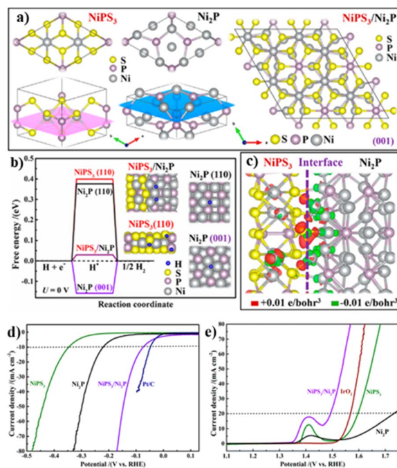
Fig. 3 (a) Graphical models to show the lattice match between NiPS 3 and Ni 2 P; (b) \Delta G_{\text{H}^*} calculation; (c) charge density distribution at the interface, The Ni, S, P, and H atoms are marked in gray, yellow, purple, and blue, respectively; LSV curves of (d) HER and (e) OER. Reproduced with permission from ref. 44. © American Chemical Society, 2019.
