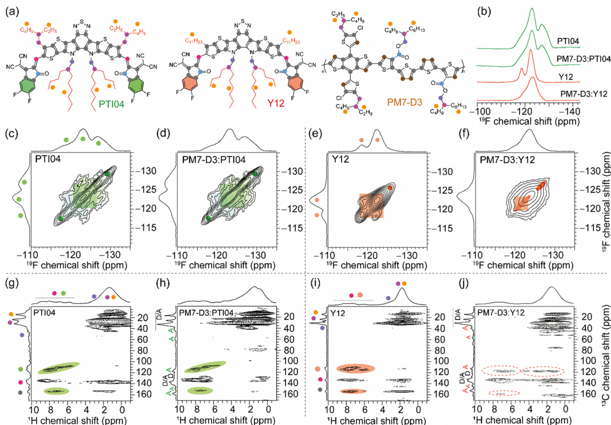
Fig. 5 (a) Structures of PM7-D3 , PTI04 , and Y12 with color dots to guide the analysis of 2D NMR spectra. (b) Solid-state 1D ^{19}\text{F} MAS NMR spectra of PTI04 and PM7-D3:MA blends. Solid-state 2D ^{19}\text{F} - ^{19}\text{F} spin-diffusion NMR spectra of (c) neat PTI04 and (d) PM7-D3:PTI04 indicating the identical acceptor morphology, and (e) neat Y12 and (f) PM7-D3:Y12 blend films with different peak patterns highlighted in red. Solid-state 2D ^1\text{H} - ^{13}\text{C} HETCOR NMR spectra of (g) neat PTI04 and (h) PM7-D3:PTI04 indicating the identical local acceptor morphology as depicted by green ovals, and (i) neat Y12 and (j) PM7-D3:Y12 BHJ blend films showing the difference in the local morphology as depicted in the red dashed ovals.
