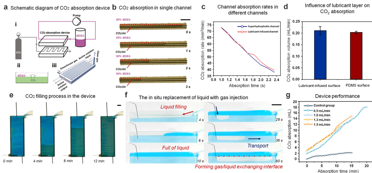
Fig. 4 CO 2 absorption with a SLISO channel-based microchip. (a) The process of on-chip CO 2 capture. The amine solution is circulated on the upper side and the CO 2 /air mixture is continuously injected on the lower side (i), where the CO 2 is continuously absorbed by the amine solution at the gas-liquid interface (ii). (iii) Schematic diagram of the gas/liquid exchanging microchip with continuous SLISO folded channels. (b) The process of absorption of the CO 2 /air mixture in a SLISO hierarchical gas channel immersed in 50% MDEA solution, scale bar = 1 cm. (c) The speed of reduction in the volume of the CO 2 /air mixture column in the SLISO hierarchical channel and the superhydrophobic channel immersed in 50% MDEA solution, which can be shown without significant differences. (d) Absorption speed of CO 2 bubbles on the lubricant-infused surface and PDMS surface immersed in 50% MDEA solution. (e) The process of filling the CO 2 absorbing device with CO 2 gas. Scale bar 1 cm. (f) Demonstration of the process of injecting a bright blue stained amine solution in a single channel until it is full, then injecting CO 2 gas forward transport. The gas/liquid interaction process in the integrated CO 2 absorption device is similar to this. Scale bar = 1 cm. (g) The effect of CO 2 gas injection rate on the absorption rate of CO 2 absorption devices. The control group is the hollow microchip without a SLISO hierarchical channel. The result shows that the gas injection rate has little effect on the absorption rate of the devices due to the fast balance of CO 2 absorption. In contrast, the presence of channels has an obvious effect on the absorption rate of the devices, which indicates that the main factor affecting the absorption rate of CO 2 absorption devices is the gas/liquid contact area.
