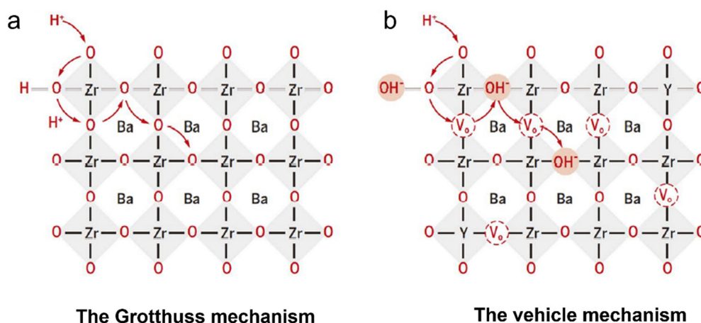
Fig. 2 Schematics of two \text{H}^+ conducting mechanisms in a \text{BaZrO}_3 -based perovskite oxide: (a) the Grotthuss mechanism and (b) the vehicle mechanism. 17
