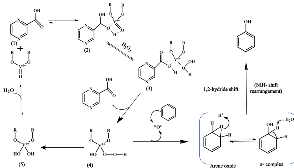
Scheme 21 Proposed reaction mechanism for the formation of vanadium-PCA complex in H 2 O 2 (aq)-CH 3 CN system (R = bulk VO x ).
