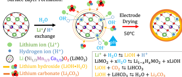
Fig. 2 When the NMC material is exposed to water \text{Li}^+ starts leaching out from its structure while \text{H}^+ from the water intercalates with the structure. 44 \text{OH}^- in the solution steadily increases the pH and combines with \text{Li}^+ to form \text{LiOH} as the water evaporates during electrode drying. Furthermore, \text{LiOH} reacts with \text{CO}_2 to form \text{LiHCO}_3 and eventually \text{Li}_2\text{CO}_3 .
