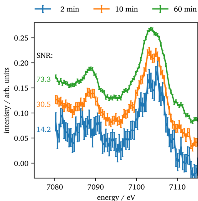
Fig. 8 Vtc spectra of Fe 2 O 3 at 75 GPa for different integration times. The SNRs are calculated for the maximum of the K \beta_{2,5} emission with the background averaged between 7100 eV and 7110 eV. The data have been offset by 0.05 units for clarity.
