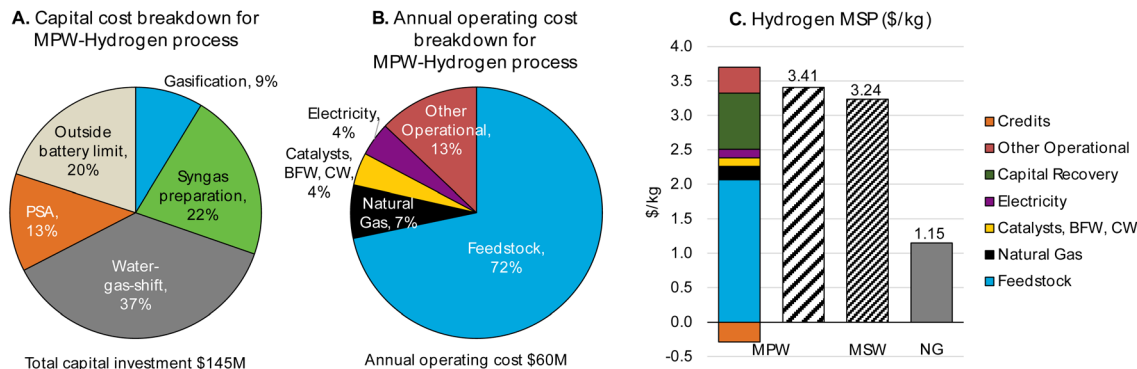
Fig. 5 CAPEX, OPEX, and MSP breakdown for MPW-hydrogen process (MPW: 240 MT per D feedstock, 70 MT per D hydrogen). (A) Detailed breakdown of CAPEX by process section is given in Table S12. † (B) A detailed breakdown of OPEX for variable and fixed costs is given in Table S13. † (C) A comparison of MSP for MPW-Hydrogen, MSW-hydrogen, and natural gas (NG)-based processes. The breakdown and net MSP for the MPW-hydrogen process are shown in separate bars. In the MSW-hydrogen case, the feedstock cost is zero. A detailed MSP breakdown by process section is given in Table S14. †
