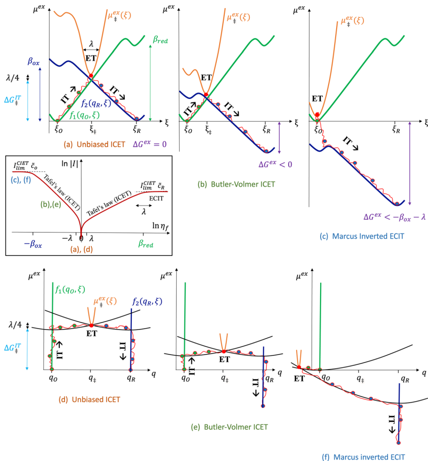
Fig. 7 Physics of IT-limited non-adiabatic CIET, or "ion-coupled electron transfer" (ICET), at a metal electrode, where the ion transfer barrier, \Delta G_{IT}^{\ddagger} , exceeds the reorganization energy \lambda , thermal energy k_B T and chemisorption function, \Delta_e . In this limit, the path of the reaction complex (red) is shown in the two dimensional landscape of excess chemical potential \mu^{ex}(q, \xi) , shown in Fig. 5, viewed along the IT coordinate \xi from the oxidized state \xi_O to the reduced state \xi_R , in (a)–(c), and the dependence on the ET solvent reorganization coordinate q is shown for the same cases in (d)–(f). The oxidized state has IT energy f_1(q_O, \xi) (green), and the reduced state has IT energy f_2(q_R, \xi) (blue). The CIET barrier is \mu_{\ddagger}^{ex}(\xi) = \mu^{ex}(q_{\ddagger}, \xi) (orange). Three cases are depicted for the excess chemical potential applied between the reduced and oxidized states, \Delta G^{ex} = e\eta_f + \varepsilon_f - \varepsilon , which is the sum of the formal overpotential \eta_f and the electron energy \varepsilon below the Fermi level \varepsilon_f , sampled from the band structure of the electrode \rho_e(\varepsilon) according to the Fermi–Dirac distribution \tilde{n}_e(\varepsilon) : in (a) and (d) for unbiased ICET with \Delta G^{ex} = 0 , the rate limiting process is IT (with a large barrier \beta_{ox} (in the reduction direction) in addition to the small ET barrier \lambda/4 (light blue). In (b) and (e) for moderate overpotentials, \Delta G^{ex} < 0 , Butler–Volmer kinetics holds for ICET. In (c) and (f) at even larger driving force, \Delta G^{ex} < -\beta_{ox} - \lambda , the reaction complex enters the Marcus inverted region of ECIT, as the ion sits at the oxidized state before ET triggers IT to complete the reaction. (Inset) Tafel plot showing the scenarios (a)–(c) for reduction, where the Tafel slope is \alpha_{IT} = \beta_{red}/(\beta_{red} + \beta_{ox}) for the negative reduction branch and 1 - \alpha_{IT} for the positive oxidation branch. On both sides, the straight-line Tafel regime transitions to a reaction limited current for Inverted ECIT, when the overpotential exceeds the ion-transfer energy.
