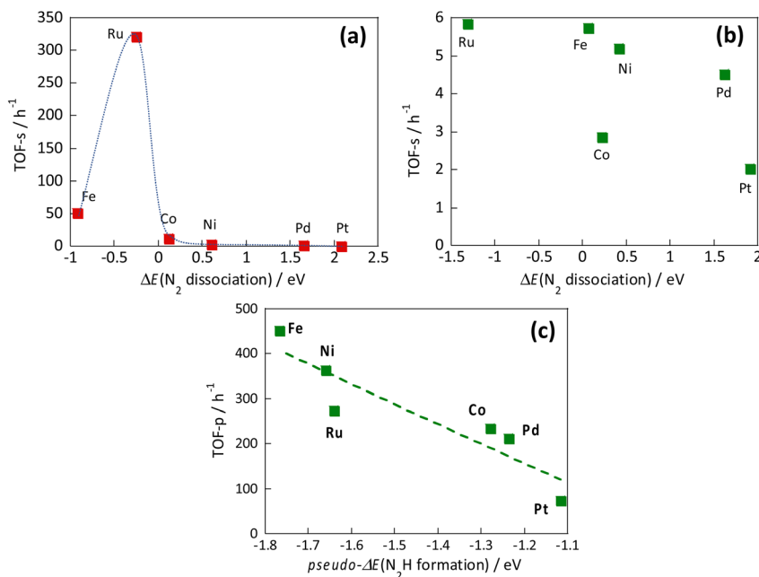
Fig. 13 Correlation between the N_2 dissociation energy and the TOF-s of the catalytic reaction upon heating (a), correlation when the electric field is applied (b), and correlation between N_2H formation energy and TOF-p (c). 36
