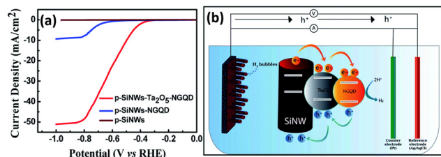
Fig. 20 (a) PEC HER performance of the p-SiNWs-Ta 2 O 5 -NGQD photoelectrodes. (b) Schematic diagram of the charge transfer process in the p-SiNWs-Ta 2 O 5 -NGQD photoelectrode. Reproduced with permission from ref. 141, Copyright © The Royal Society of Chemistry 2022.
