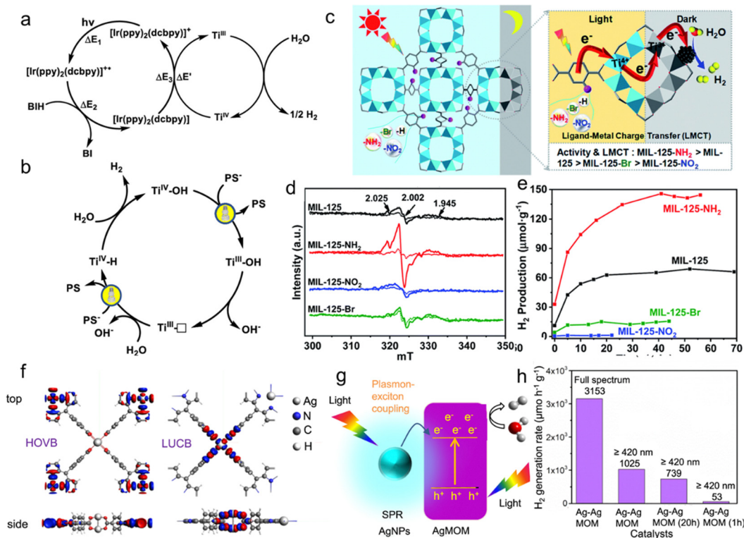
Fig. 5 (a) Proposed Catalytic Cycle for the Visible Light-Driven HER Catalyzed by Ti_3 -BPDC-Ir; (b) detailed catalytic mechanism on the Ti Site via the Ti^{IV}/Ti^{III} Cycle. Reproduced with permission from ref. 90 (Copyright 2019, American Chemical Society). (c) Illustration showing the dark photocatalysis over MIL-125 and MIL-125 with different functional groups, MIL-125-X (X = NH_2 , NO_2 , Br). (d) Dark photocatalytic hydrogen production activity comparison of MIL-125 and MIL-125-X (X = NH_2 , NO_2 , Br) with 0.5 mL TEOA as a sacrificial agent at 25 °C. (e) ESR spectra (solid and dotted lines represent signals in the dark and when light is on, respectively) for MIL-125 and MIL-125-X (X = NH_2 , NO_2 , Br). Reproduced with permission from ref. 91 (Copyright 2022, The Royal Society of Chemistry) (f) DFT calculated highest occupied valence band (HOVB) and lowest unoccupied conduction band (LUCB) topologies of MOM. (g) Proposed visible-driven photocatalytic mechanism of Ag-AgMOM. (h) Hydrogen generation rate under 300 W irradiation in the presence of Ag-AgMOM synthesized at reaction time of 1 h, 20 h and 28 h with or without a 420 nm long-pass filter, respectively. Reproduced with permission from ref. 92 (Copyright 2023, Springer Nature).
