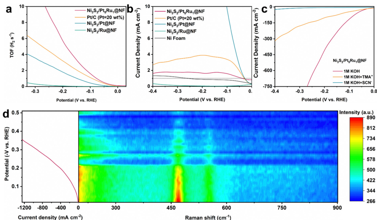
Fig. 4 Mechanism study of Ni 3 S 2 /Pt 5 Ru 1 @NF. (a) The potential-dependent TOF curves for Ni 3 S 2 /Pt 5 Ru 1 @NF, Pt/C, Ni 3 S 2 /Pt@NF and Ni 3 S 2 /Ru@NF, (b) calculated KIE values (J H 2 O /J D 2 O ) from Ni 3 S 2 /Pt 5 Ru 1 @NF, Pt/C, Ni 3 S 2 /Pt@NF, Ni 3 S 2 /Ru@NF and Ni foam, (c) polarization curves for Ni 3 S 2 /Pt 5 Ru 1 @NF before and after the addition of SCN - and TMA + ions in N 2 -saturated 1.0 M KOH, and (d) operando Raman spectra of Ni 3 S 2 /Pt 5 Ru 1 @NF in 1.0 M KOH under HER potential.
