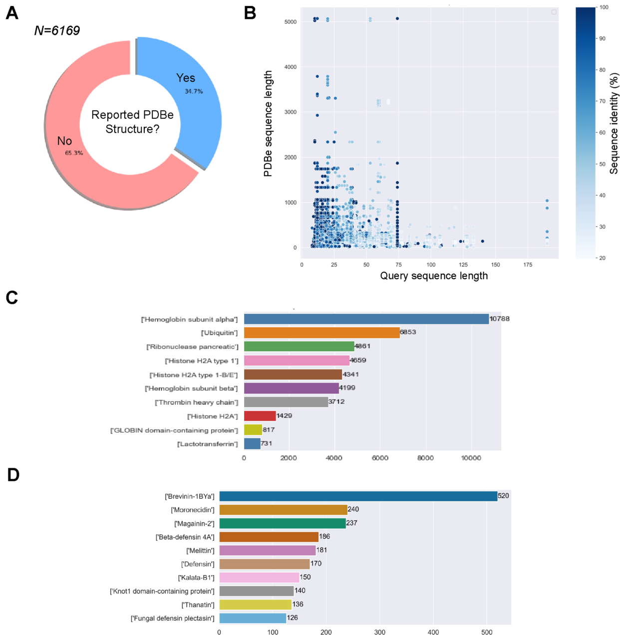
Fig. 1 Obtaining our benchmarking dataset of GRAMPA sequences and related PDBe structures. (A) Percentages of GRAMPA sequences with or without related experimental structures, (B) comparing length and identity between GRAMPA sequences and matching PDBe sequences, (C) peptides or proteins with the largest number of related GRAMPA sequences, and (D) most represented AMP families after filtering the repository.
