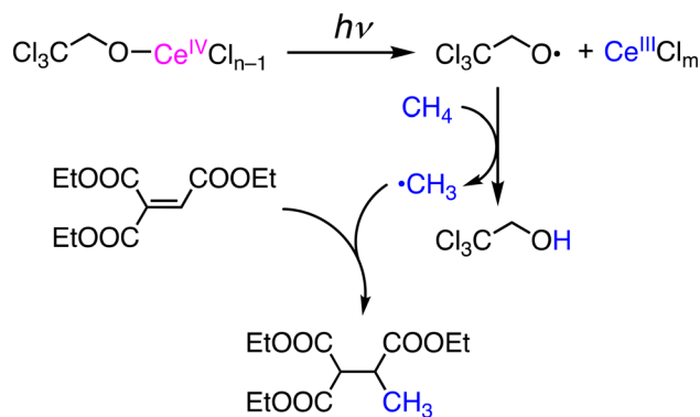
Scheme 11 Photoinduced functionalization of CH 4 based on LMCT in a Ce IV –alkoxo complex to generate an alkoxo radical. 33
