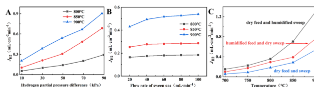
Fig. 6 H 2 permeation performance of BCYF 0.10 -YDC/BCYF 0.10 -Ni double layer HF membranes at: (A) different H 2 partial pressure difference (feed gas was 100 mL min -1 of H 2 /He mixture and sweep gas was 100 mL min -1 of N 2 ); (B) different sweep gas flow rate (feed gas was 100 mL min -1 of 50 vol% H 2 /He mixture); (C) different humid atmospheres (feed gas was 100 mL min -1 of room-temperature steam saturated 50 vol% H 2 /He mixture and sweep gas was 100 mL min -1 of N 2 ).
