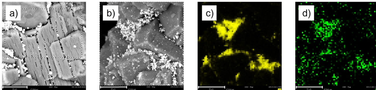
Fig. 11 SEM images of (a) SCALMS-C and (b) SCALMS-C* and EDX mapping of SCALMS-C* showing (c) gallium and (d) platinum. The scale bar represents 10 \mu\text{m} .
