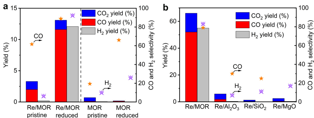
Fig. 3 POM over different catalysts. (a) \text{Re}/\text{MOR} and \text{MOR} before and after \text{H}_2 reduction ( 600^\circ\text{C} ). Reaction conditions: 600^\circ\text{C} , \text{CH}_4:\text{O}_2:\text{N}_2 = 50:4:46 , space velocity (SV) of 60\,000\text{ mL g}^{-1}\text{ h}^{-1} . (b) Effect of catalyst support. Catalysts were reduced before POM. 600^\circ\text{C} , \text{CH}_4:\text{O}_2:\text{N}_2 = 8:4:88 , SV of 12\,000\text{ mL g}^{-1}\text{ h}^{-1} . All the data in (a) and (b) are results at 1 h after starting the reaction.
