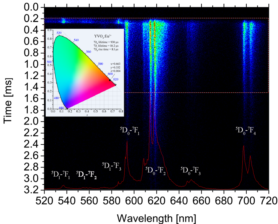
Fig. 6 Typical time-resolved spectrum of rare earth doped phosphor ( \text{YVO}_4:\text{Eu}^{3+} ) acquired in our measurements. Europium transitions are denoted. Inset shows CIE plot (color coordinate diagram) calculated from spectral data.
