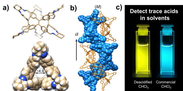
Fig. 4 (a) Views of TPE-based triangular prismatic enantiomers, self-assembling into supramolecular double helices. (b) changes in the colour of the emission from blue to yellow to traces of acids in organic solvents. (c) reproduced and adapted with permission from J. Mater. Chem. C , 2022, 10 , 15394. 66
