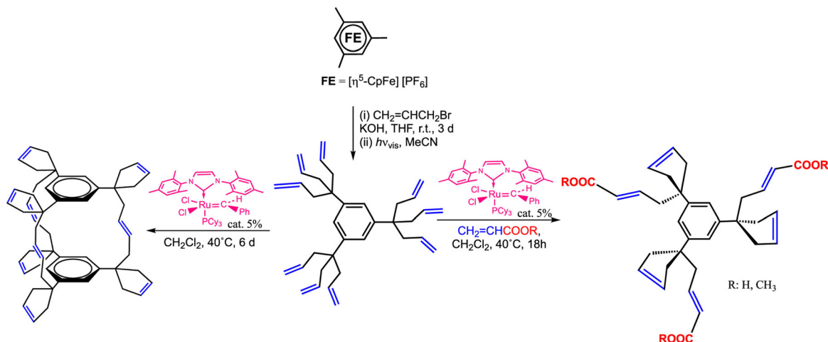
Scheme 14 Single-pot \text{CpFe}^+ -induced nona-allylation of mesitylene followed by olefin metathesis reaction of the 9 terminal double bonds catalyzed by the 2 nd -generation Ru Grubbs catalyst: cyclophane cage synthesis (left) or cyclization of two tethers of each tripod along with functionalization of the 3 rd one in the presence of acrylic acid or acrylate (right). Adapted with permission of ref. 140. Copyright 2008 American Chemical Society.
