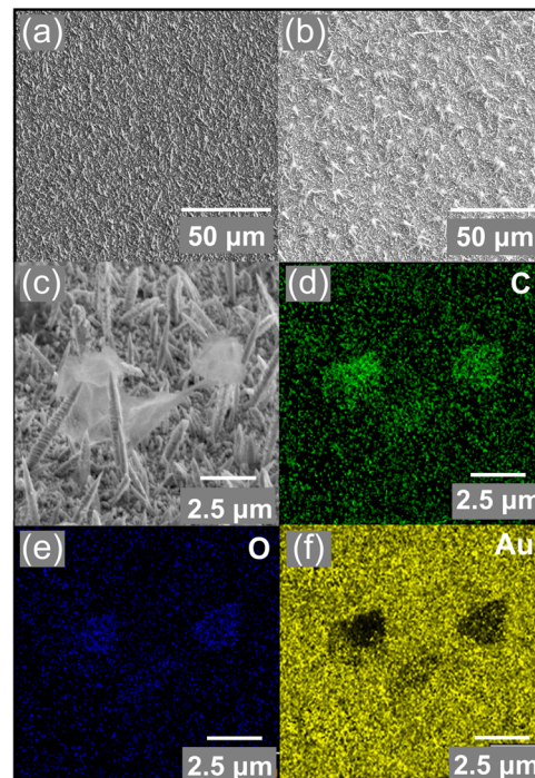
Fig. 2 FE-SEM images of the surface of the extended-gate Au electrode functionalized with (a) the AuNS layer and (b and c) the GO and AuNS layer. EDX-mapping images of (d) C, (e) O, and (f) Au for (c).
