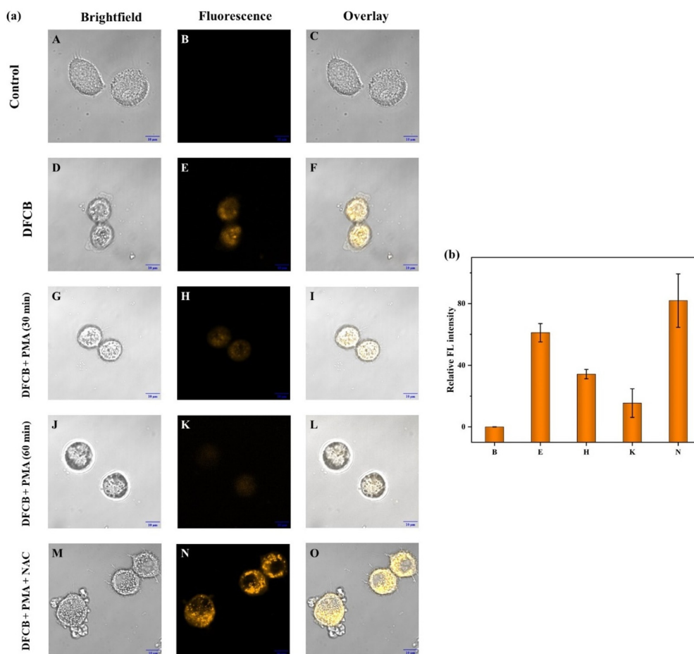
Fig. 9 (a) Imaging of H_2O_2 in HeLa cells: (A–C) HeLa cells alone were cultured for 1 h and acted as the control; (D–F) HeLa cells supplemented with the DFCB sensor ( 4 \mu M ) were cultured for 1 h; (G–I) the HeLa cells supplemented with PMA ( 1 \mu g ml^{-1} ) were cultured for 30 min; (J–L) subsequently, the HeLa cells supplemented with PMA ( 1 \mu g ml^{-1} ) were cultured for 60 min; and (M–O) the HeLa cells were cultured with PMA ( 1 \mu g ml^{-1} ) and then incubated with NAC ( 1 mM ), followed by staining with the DFCB sensor ( 4 \mu M ) for 1 h. (b) The quantitative intensity was obtained from the fluorescent images of the HeLa cells.
