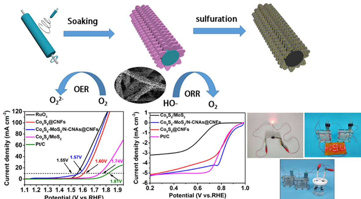
Fig. 18 Schematic representation of the preparatory scheme of \text{Co}_9\text{S}_8\text{-MoS}_2/\text{NCNAs}@ \text{CNFs} (a). Polarisation curve with the pictorial representation of the circuit (b). Reproduced from ref. 126 (Copyright 2022, American Chemical Society).
