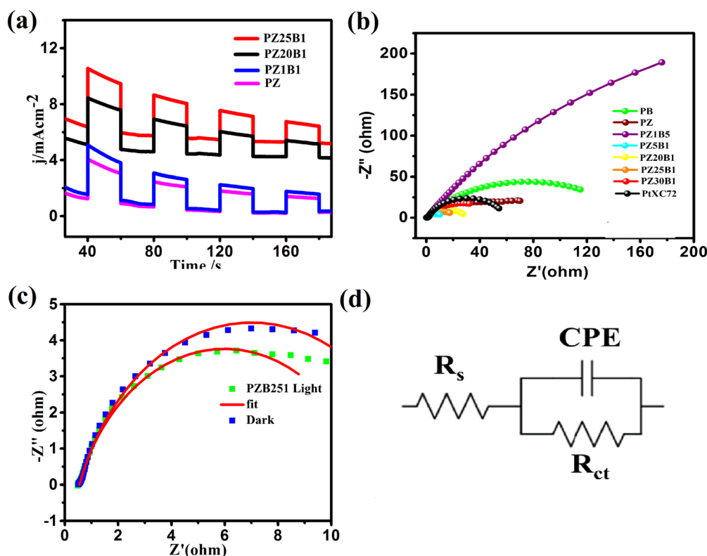
Fig. 8 (a) Photocurrent responses of PB, PZ, and different PZB composite electrodes under visible light illumination in 0.5 \text{ M MeOH} + 1 \text{ M NaOH} solution recorded at -0.3 V. (b) EIS spectra of PB, PZ, PZ5B1, PZ25B1, PZ30B1 in 0.5 \text{ M MeOH} + 1 \text{ M NaOH} solution recorded at -0.3 V with visible light exposition in the range of 0.1 - 100 \text{ Hz} . (c) Spectra of PZ25B1 electrodes with dark and light illumination. (d) Equivalent circuit of the corresponding figure.
