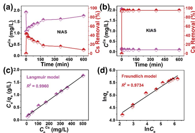
Fig. 5 (a) Adsorption kinetics for Cs^{+} by (a) unactivated NIAS and (b) KIAS plotted as concentration (mg L -1 ) (purple line) and removal rate (%) (red line) vs. time (min). (c) The Langmuir and (d) Freundlich isotherm models of Cs^{+} adsorption using KIAS.
