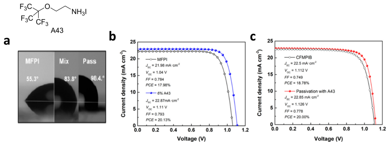
Fig. 25 (a) Water contact angle studies of pristine MFPI and A43 doped 2D/3D-films of MFPI and CFMPIB. (b) Current–voltage curves for MFPI- and A43-based 2D/3D-perovskite devices. (c) Current–voltage curves for pristine CFMPIB and A43-based 2D/3D-perovskite devices. 31 Reproduced with permission from ref. 31. Copyright 2018, American Chemical Society.
